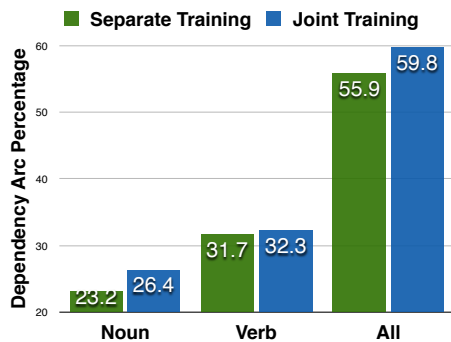
Figure 1: Percentages of dependencies satisfying linguistic rules in the LC-DMV parses of the English test dataset. Noun and Verb denote dependencies headed by nouns and verbs.
